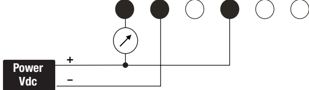
3 Wire 4-20 mA Output V+ V- Vout EXT S1 S2
